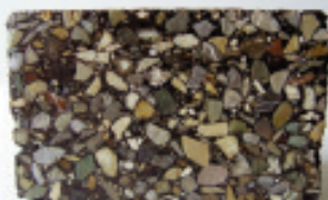
Splittmastixasphalt 0/8S ZTV Asphalt
